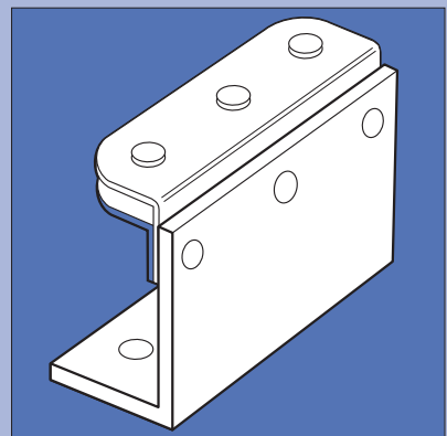
Return pulley assembly
